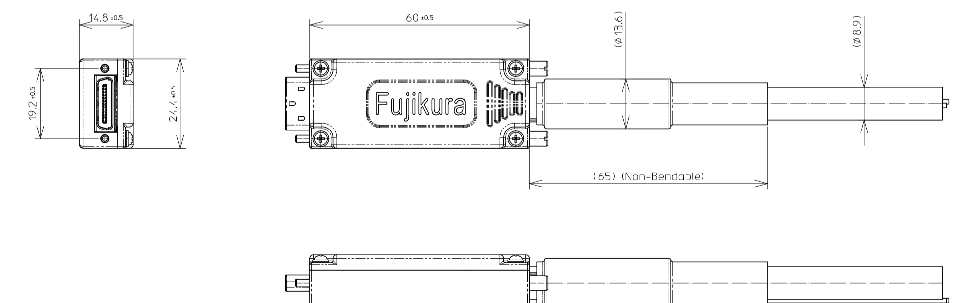
Grabber Side SDR with Power Supply
