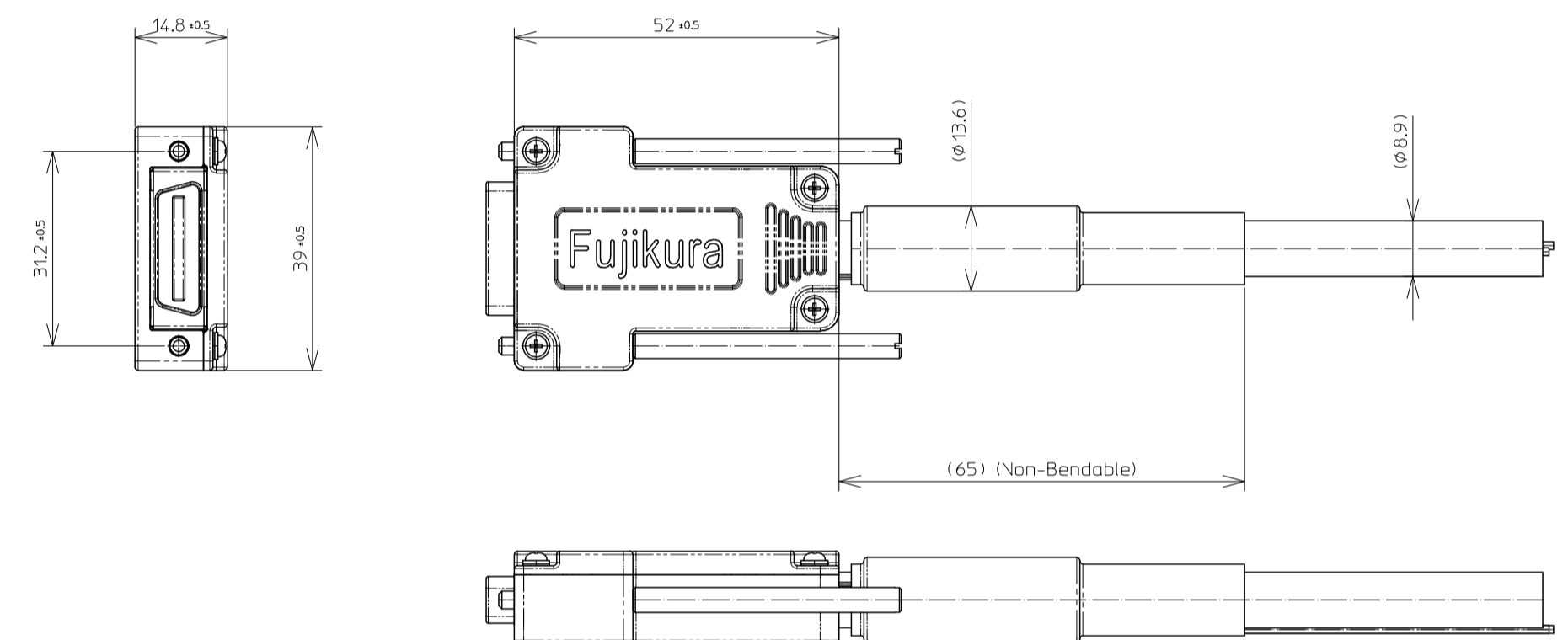
Grabber Side MDR with Power Supply
